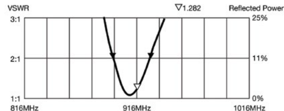
The Linx ANT-916-CW-HWR-SMA antenna is used for 908...917, 919...921 MHz (ZMEURAZBERRY7_ANT)
