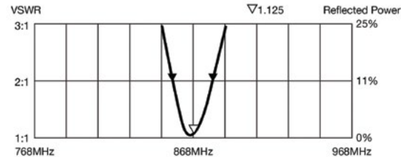
The Linx ANT-868-CW-HWR-SMA antenna is used for 865...869 MHz (ZMEERAZBERRY7_ANT)
